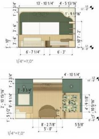
Figure 7. Perspective, elevations, floor plan and ceiling plan of the nurse's station created by A. C.
