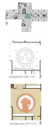
Figure 7. Perspective, elevations, floor plan and ceiling plan of the nurse's station created by A. C.
